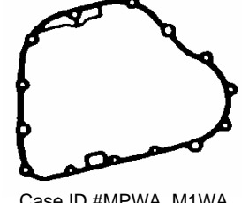
Case ID #MPWA, M1WA Case gasket, 2 Shaft Part #48937 Kit #K48900V, K48900W Car type 1992-94 Vigor, 1995-98 2.5TL OEM #21811-PW7-000
