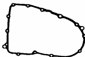
HM-3 Speed Case gasket Part #48704A Kit #K48900X Car type 1980-82 Accord, 1980-82 Prelude, 1981-83 Civic OEM #21811-PA9-020
