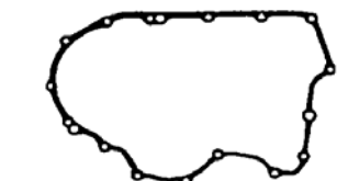
Case ID #B6VA, M6HA, BAXA, MAXA, MDWA Case gasket, 3 Shaft Part #48737B Kit #K48900D/K48900Z Car type 1998-99 2.3CL, 1997-01 Prelude, 1998-01 Accord, 1998 Odyssey, 1998 Isuzu Oasis OEM #21811-P6H-000 5-86206-042-0
