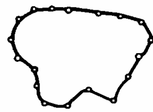
Case ID #MPZA Case gasket, 3 Shaft Part #48740 Kit #K48900S Car type 1995-97 Accord (V-6) OEM #21811-POZ-000
