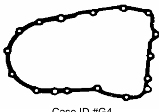
Case ID #G4 Case gasket, 2 Shaft Part #488811B* Kit #K48900T Car type 1986-87 Legend OEM #21811-PG4-010
